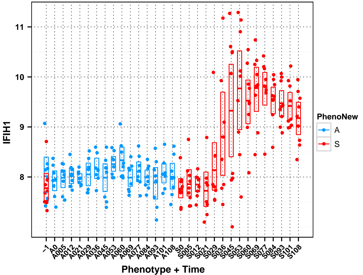
Fig. S8 Temporal gene expression of cluster 3 gene cytoplasmic double-strand viral RNA sensor IFIH1 (interferon induced with helicase C domain 1). The expression intensities are plotted on a log base 2 scale.
