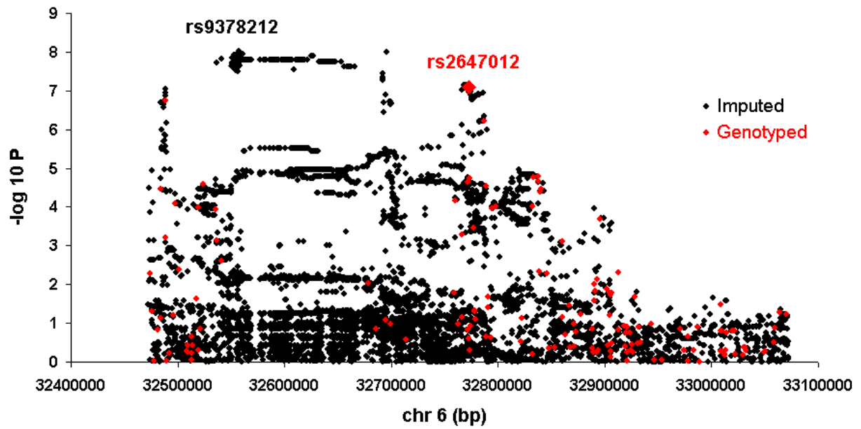
Figure S2. Association results (trend test on Stage 1, follicular lymphoma) for imputed single nucleotide polymorphism (SNPs) (black) and genotyped SNPs (red). rs9378212 is the top SNP among those showing high (>95%) concordance between HapMap and 1000 Genomes CEU genotypes.
