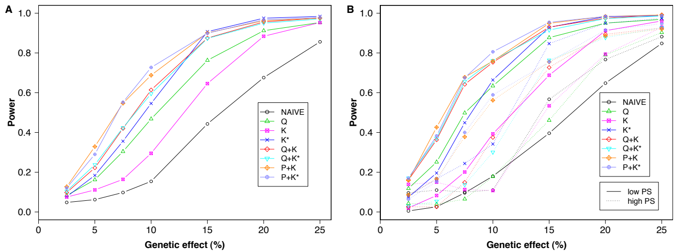
Figure S3: Power of the different methods to detect QTN using a 5% significance level, calculated as in Figure 3 but using haplotype markers. (A) Power calculated across all simulations. (B) Power calculated separately for QTN that showed strong and weak correlation with population structure.
